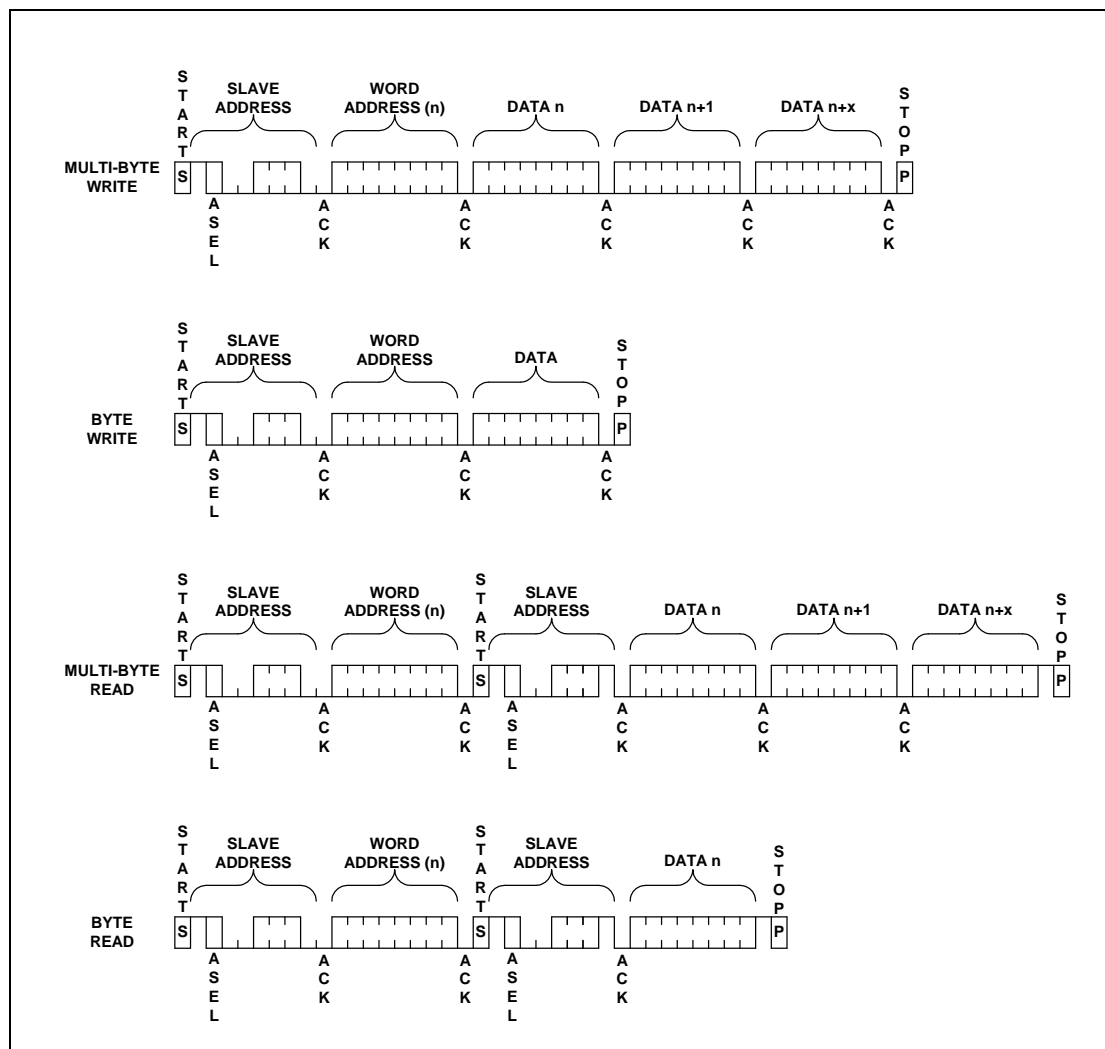
Figure 5-3. Two-Wire Serial Interface Operation
