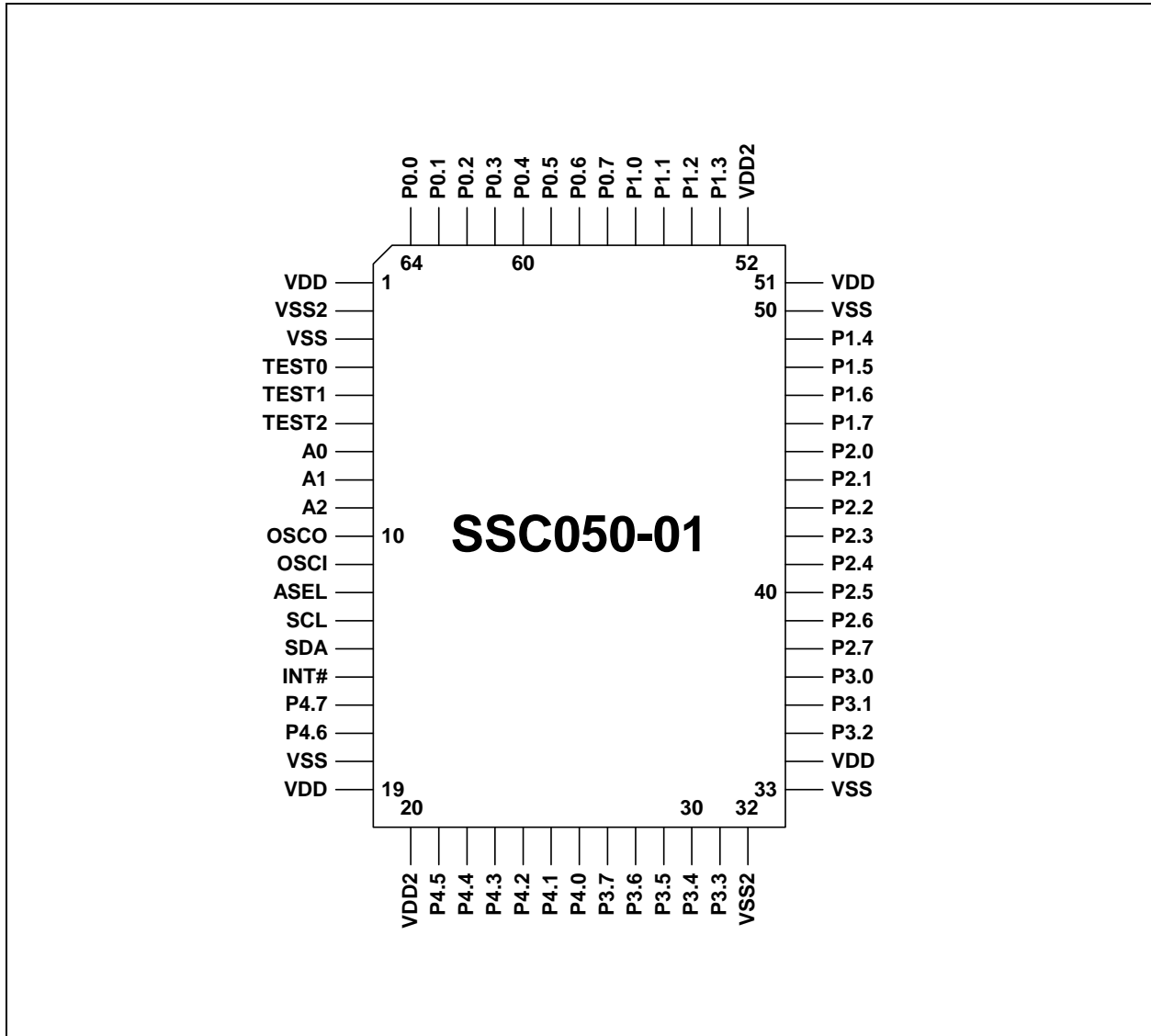
Figure 3-2. Pinout Diagram
