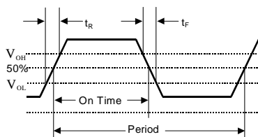
Figure 5. Output Waveform
