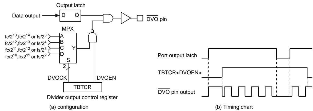
Figure 7-3 Divider Output
