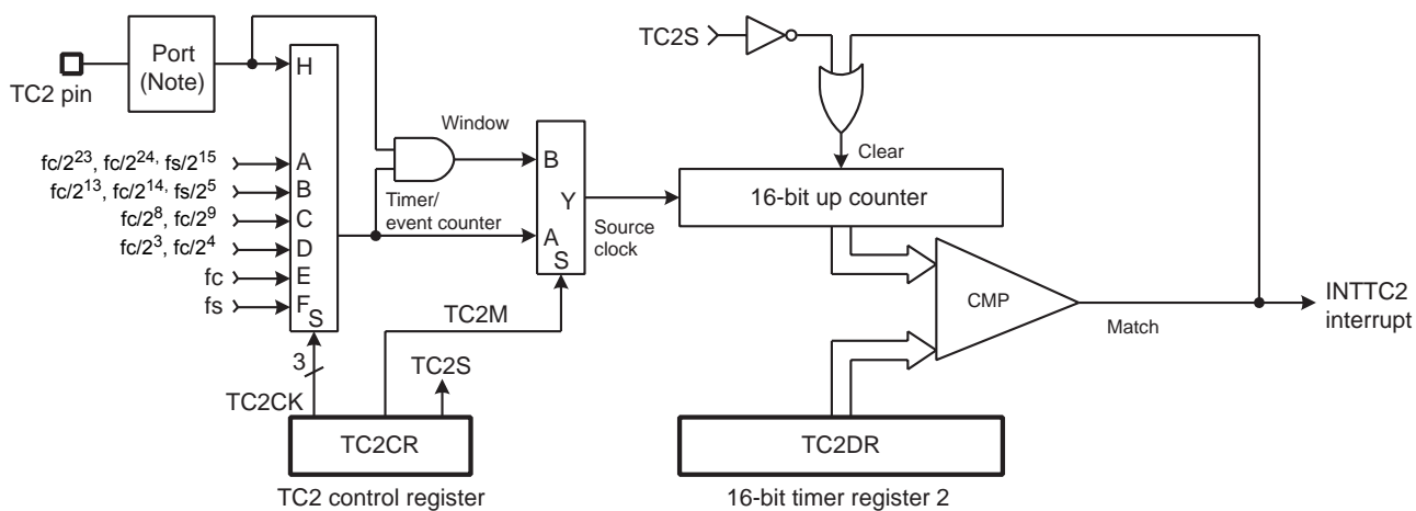
Figure 9-1 Timer/Counter2 (TC2)
