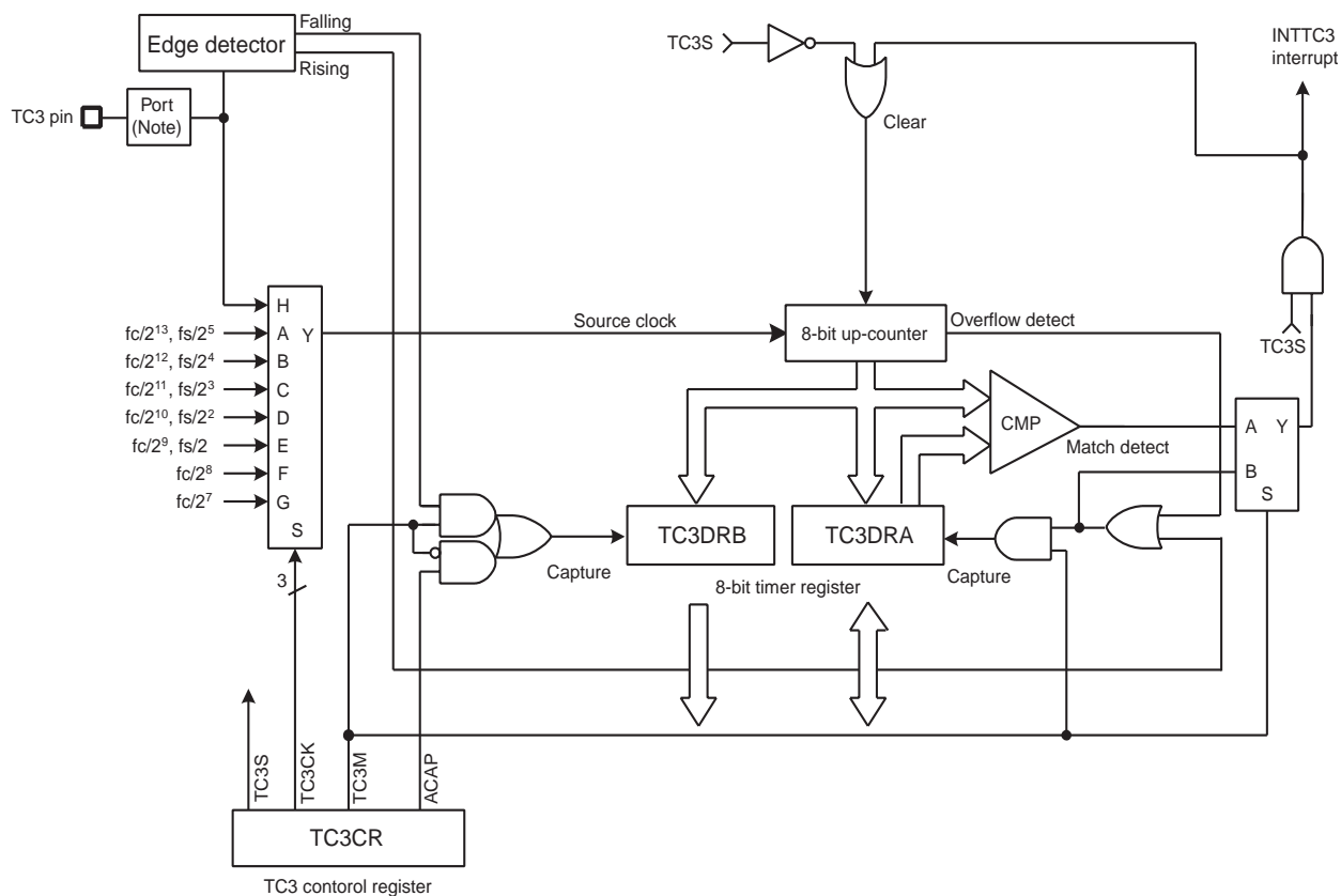
Figure 10-1 TimerCounter 3 (TC3)
