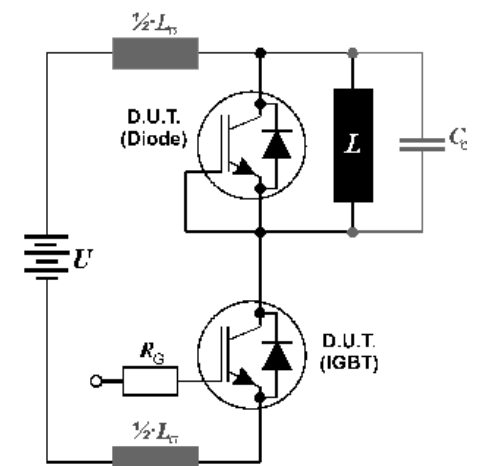
Figure E. Dynamic test circuit Leakage inductance L_{\sigma} = 180\text{nH} and Stray capacity C_g = 900\text{pF} .
