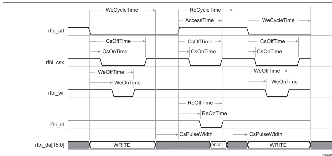
Figure 6-32. LCD Display Interface in RFB Mode – Data Read-to-Write and Write-to-Read Modes (1)(2)
