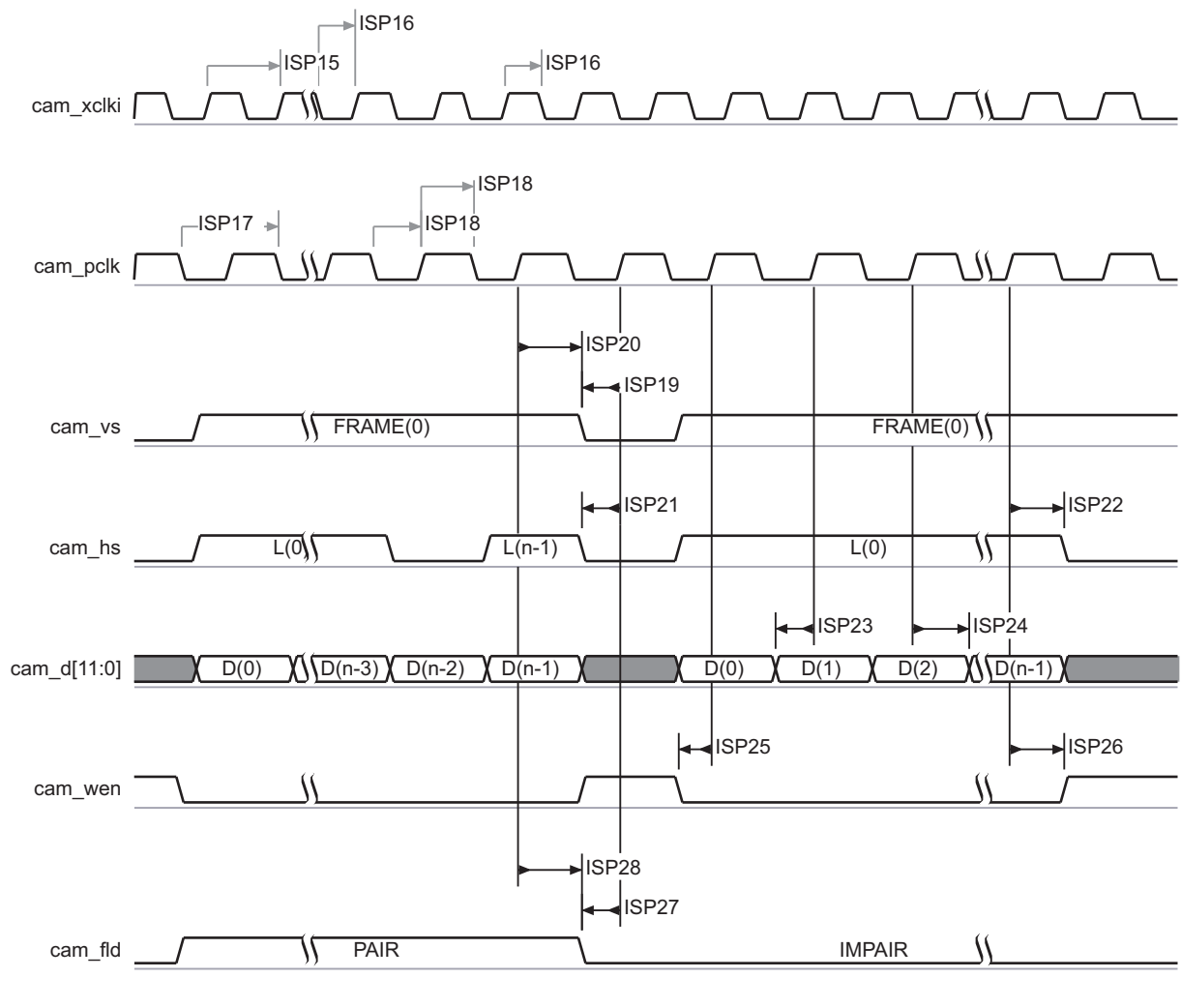
Figure 6-25. ISP – 12-Bit SYNC Normal – Interlaced Mode (1)(2)(3)(4)(5)(6)(7)(8)
