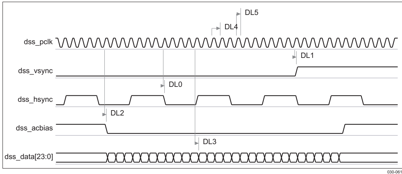
Figure 6-28. LCD Display in TFT Mode (1)(2)(3)(4)
