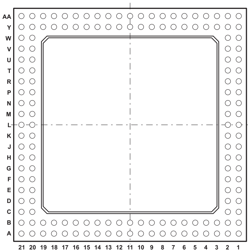
Figure 2-4. OMAP3530/25 Applications Processor CBC-SBGA-515 Package (Top View)
