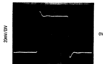
Small Signal Transient Response V_S = \pm 2.5V
