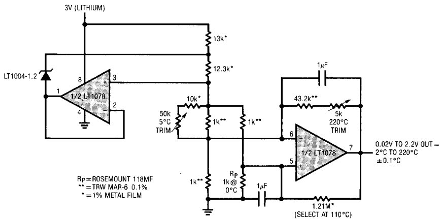
Platinum RTD Signal Conditioner with Curvature Correction
