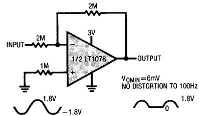
Half-Wave Rectifier
