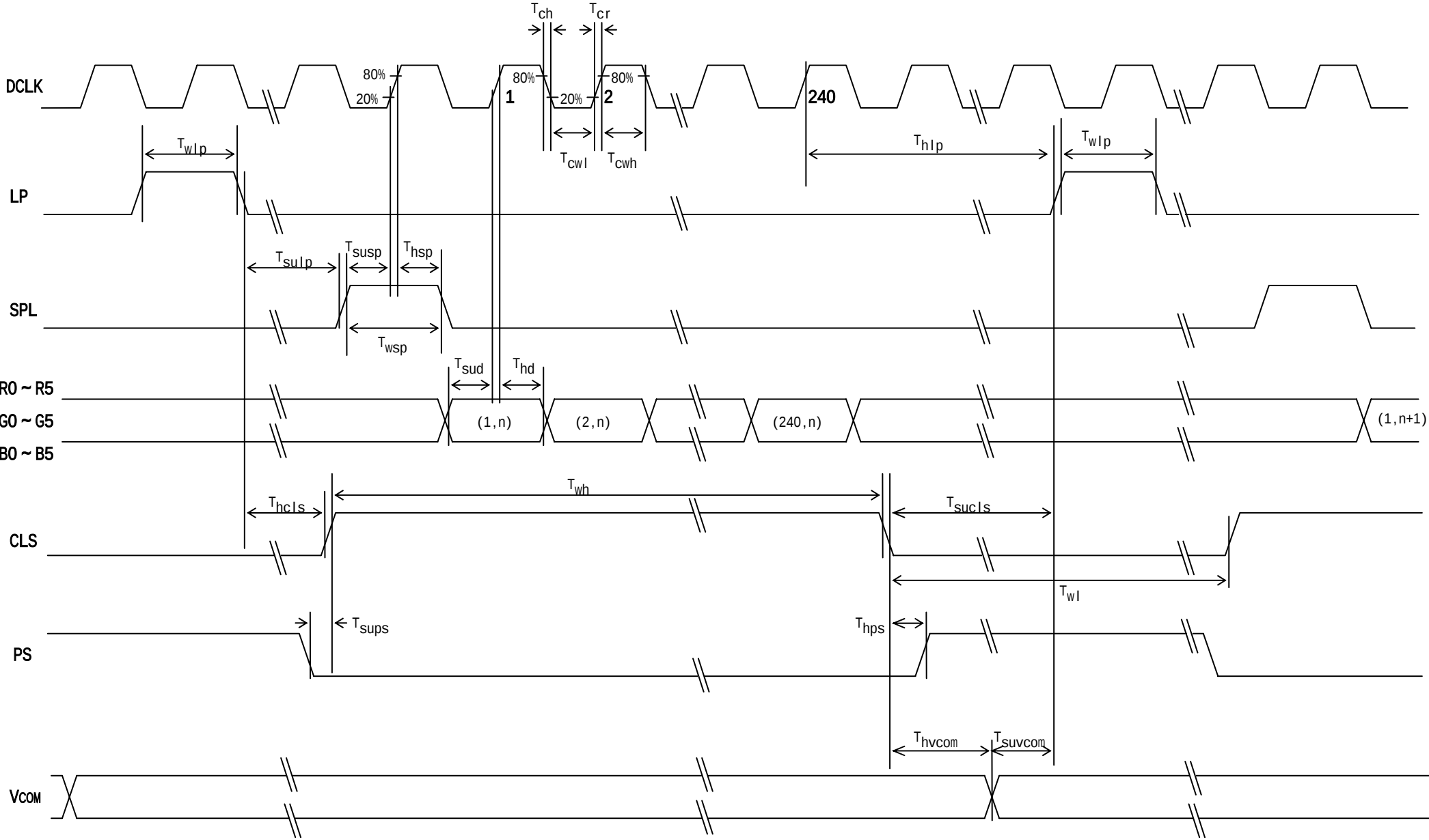
Fig.(a) Horizontal timing chart
