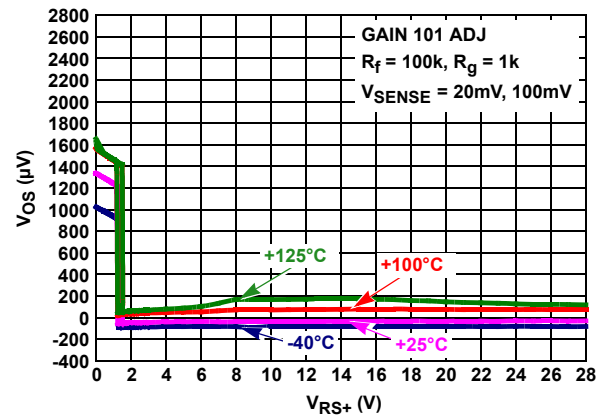
FIGURE 50. V_{OS} vs V_{RS+}
