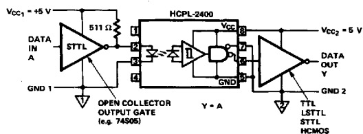
Figure 14. Alternative HCPL-2400/30 Interface Circuit.
