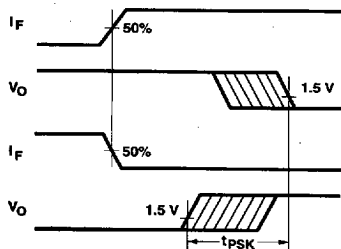
Figure 15. Illustration of Propagation Delay Skew – t_{PSK} .
