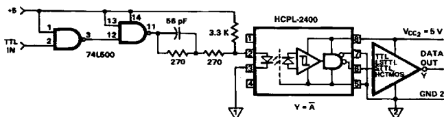
Figure 13. Recommended 20 MBd HCPL-2400/30 Interface Circuit.
