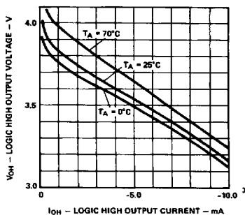
Figure 2. Typical Logic High Output Voltage vs. Logic High Output Current.
