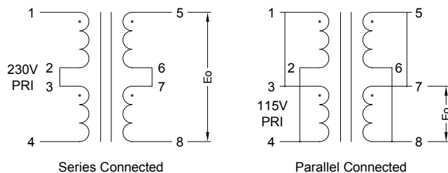
Series Connected
