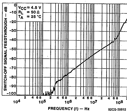
Fig. 13 - Typical switch-off signal feed through vs. frequency.
