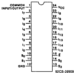
TOP VIEW TERMINAL ASSIGNMENT
