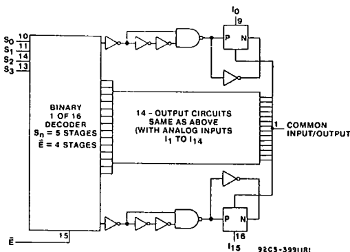
Fig. 1 - Functional diagram.
