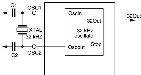
Figure 20. 32-kHz Crystal Oscillator
