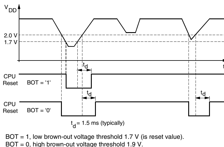
Figure 10. Brown-out Detection
