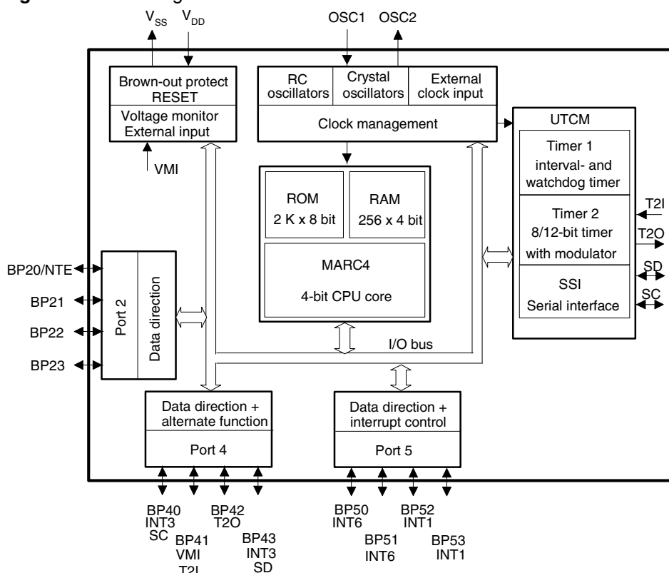
Figure 1. Block Diagram
