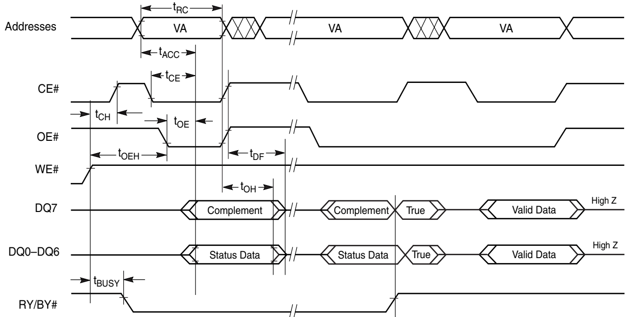
Note: VA = Valid address. Illustration shows first status cycle after command sequence, last status read cycle, and array data read cycle.
