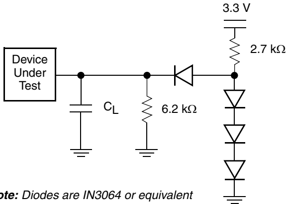
Figure 13. Test Setup
