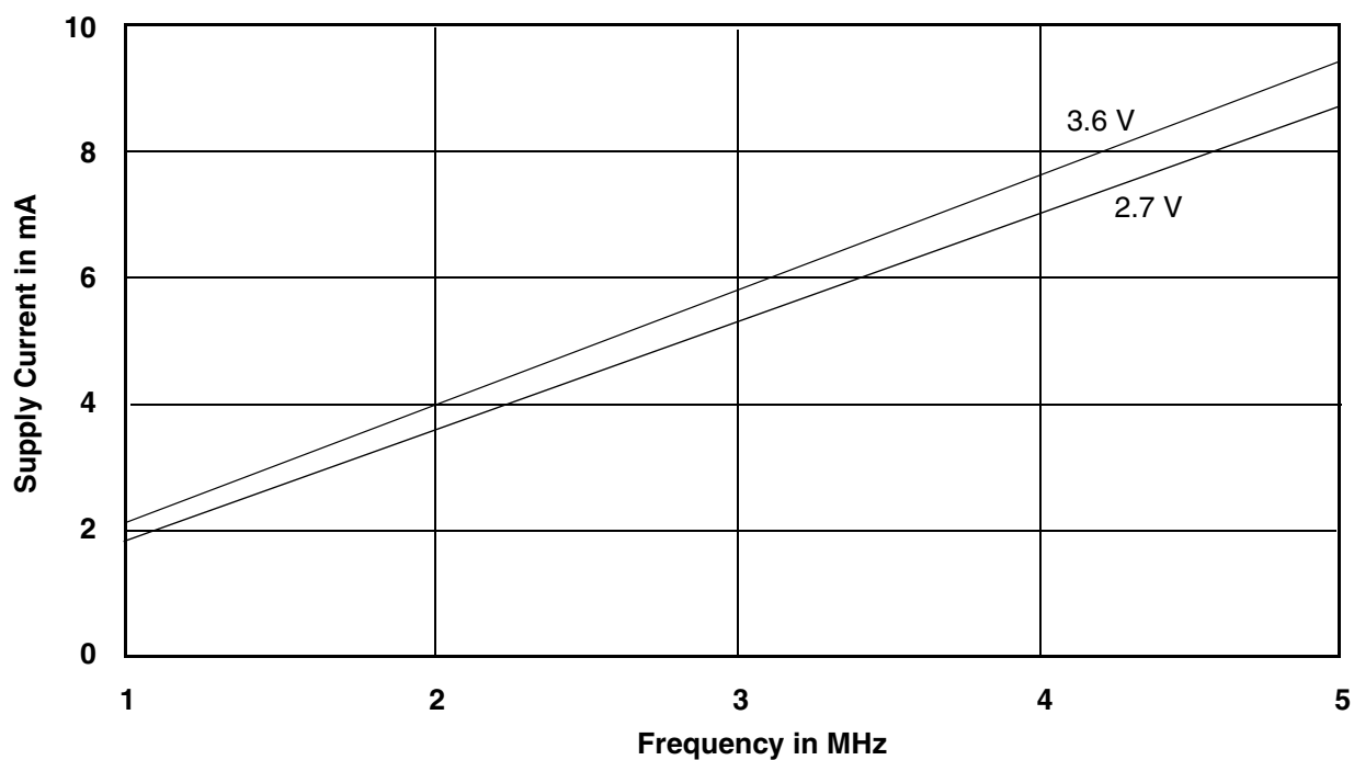
Figure 12. Typical I_{CC1} vs. Frequency
