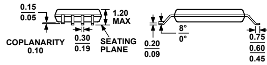
Figure 45. 8-Lead Thin Shrink Small Outline Package [TSSOP] (RU-8)
