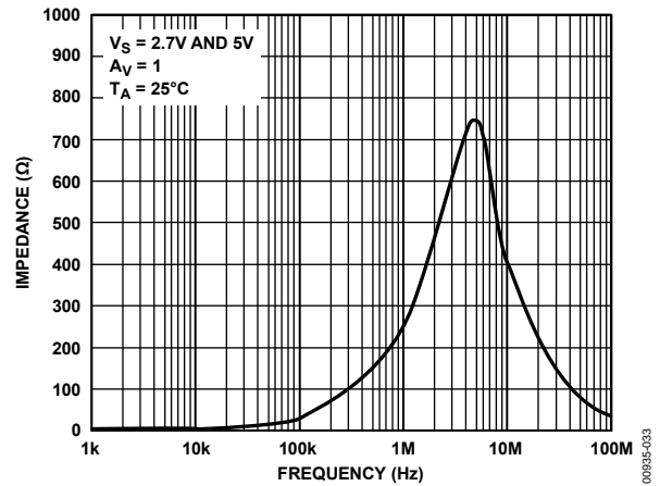
Figure 33. Closed-Loop Output Impedance vs. Frequency
