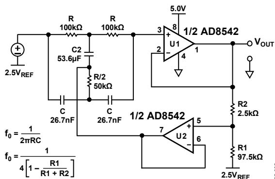
Figure 35. 60 Hz Twin-T Notch Filter, Q = 10
