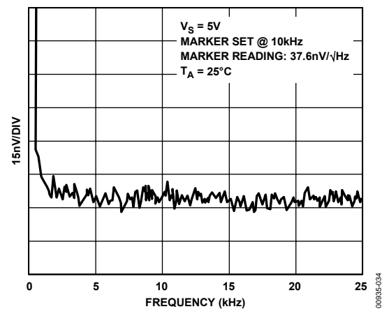
Figure 34. Voltage Noise
