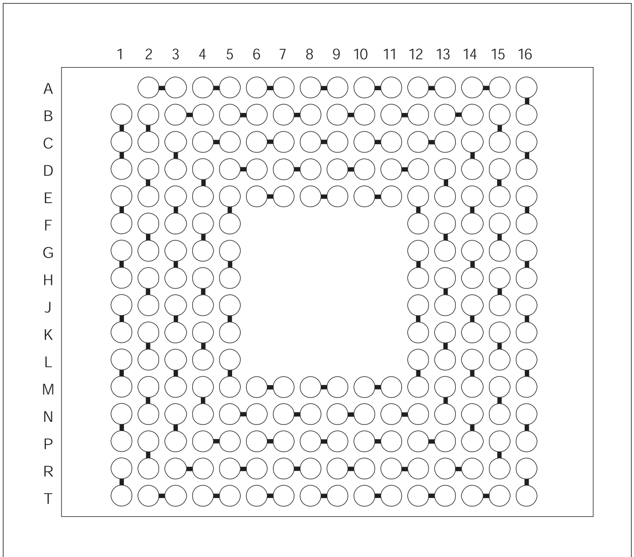
FIGURE 1 – DAISY-CHAIN INTERCONNECTION
