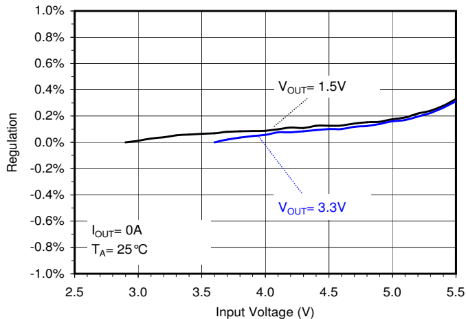
Line Regulation
