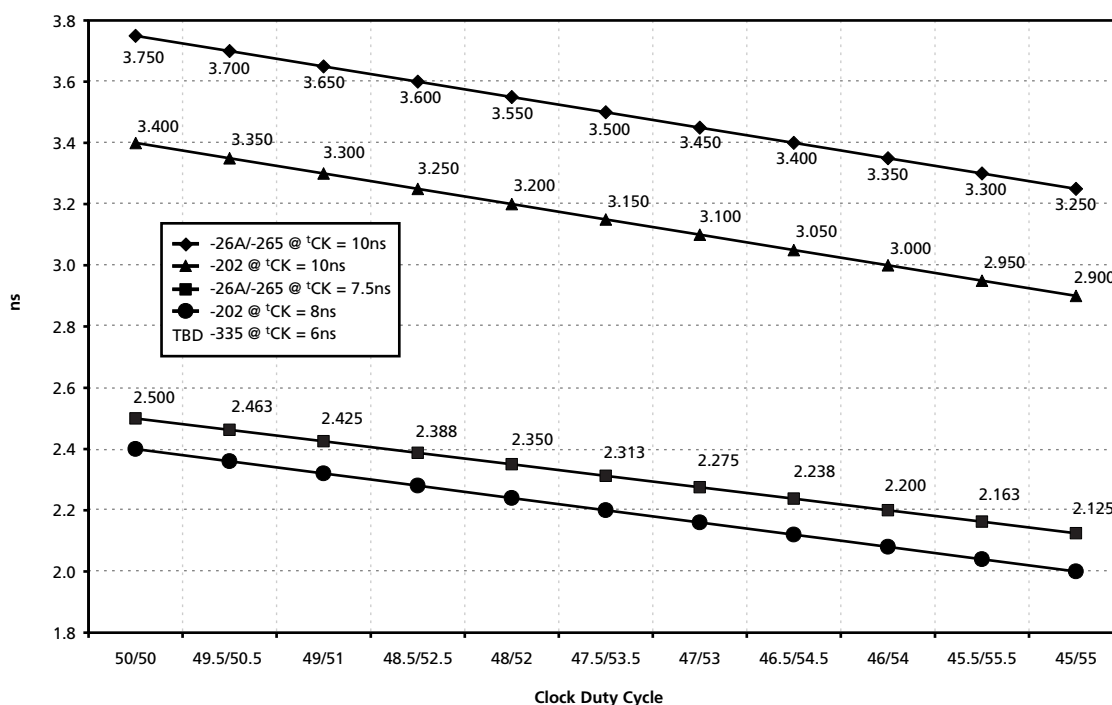
Figure 8: Derating Data Valid Window ( t_{QH} - t_{DQSQ} )
