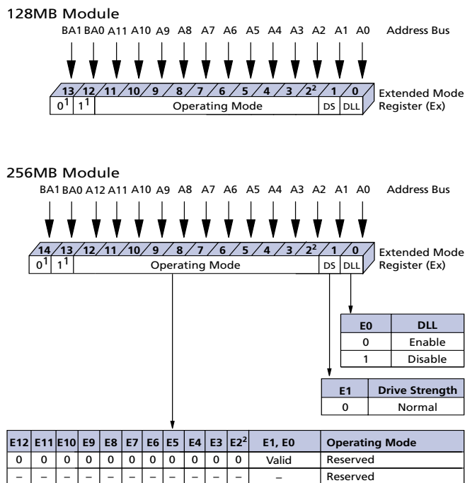
Figure 7: Extended Mode Register Definition Diagram
