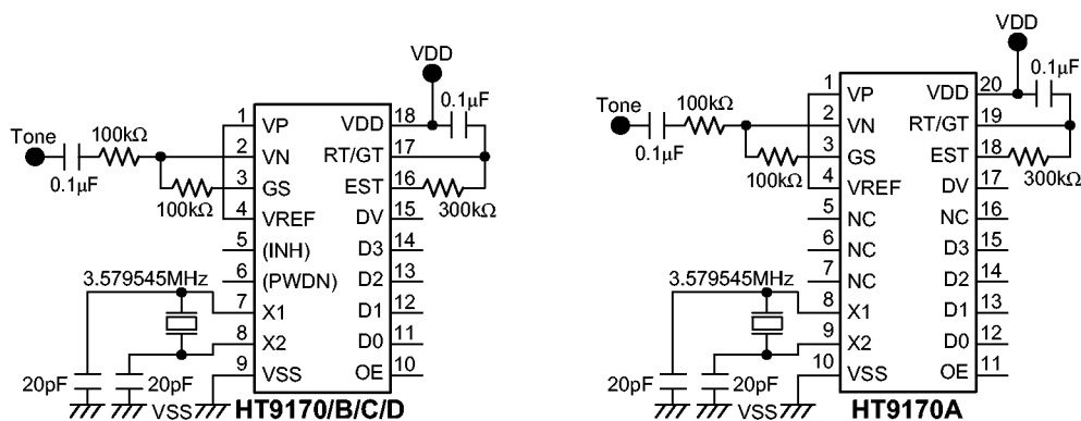
Figure 1. Test circuit
