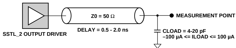
Figure 5. Test conditions for SSTL_2 output driver.
