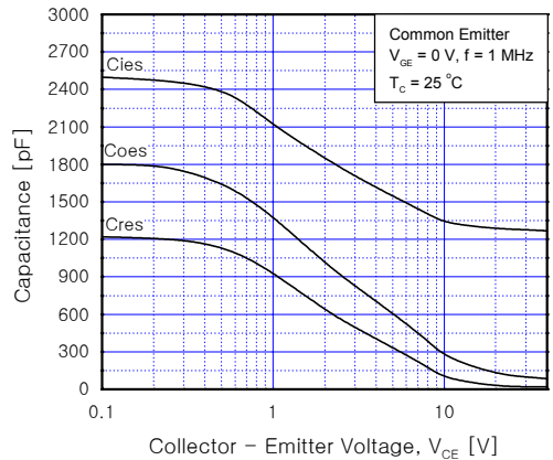
Fig 6. Capacitance Characteristics
