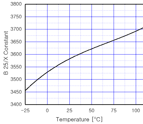
Fig 20. NTC Characteristics
