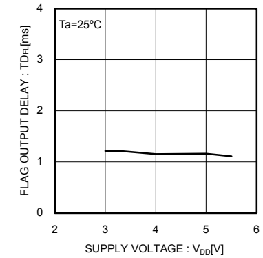
Fig.45 Flag output delay
