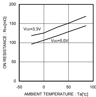
Fig.32 ON resistance
