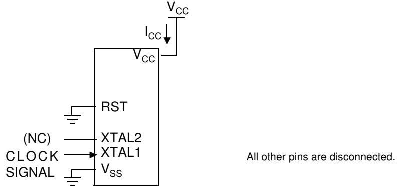
Figure 32. V_{CC} Test Condition, Under Reset
