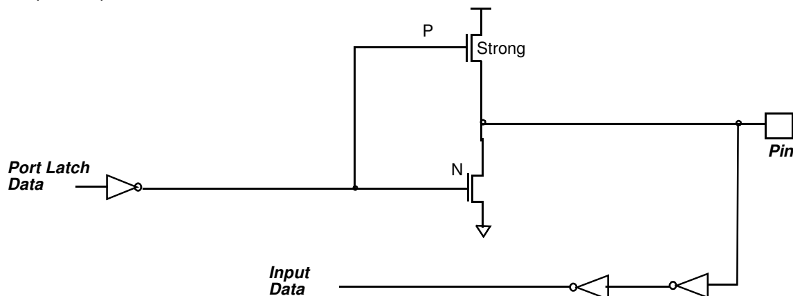
Figure 4. Push-pull Output
