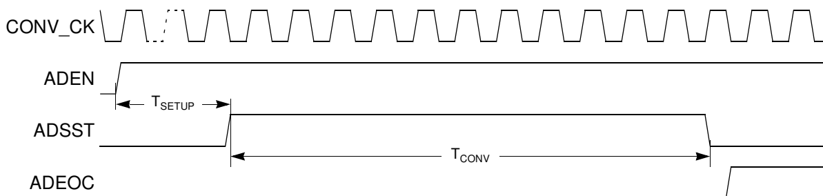
Figure 2. Timing Diagram
