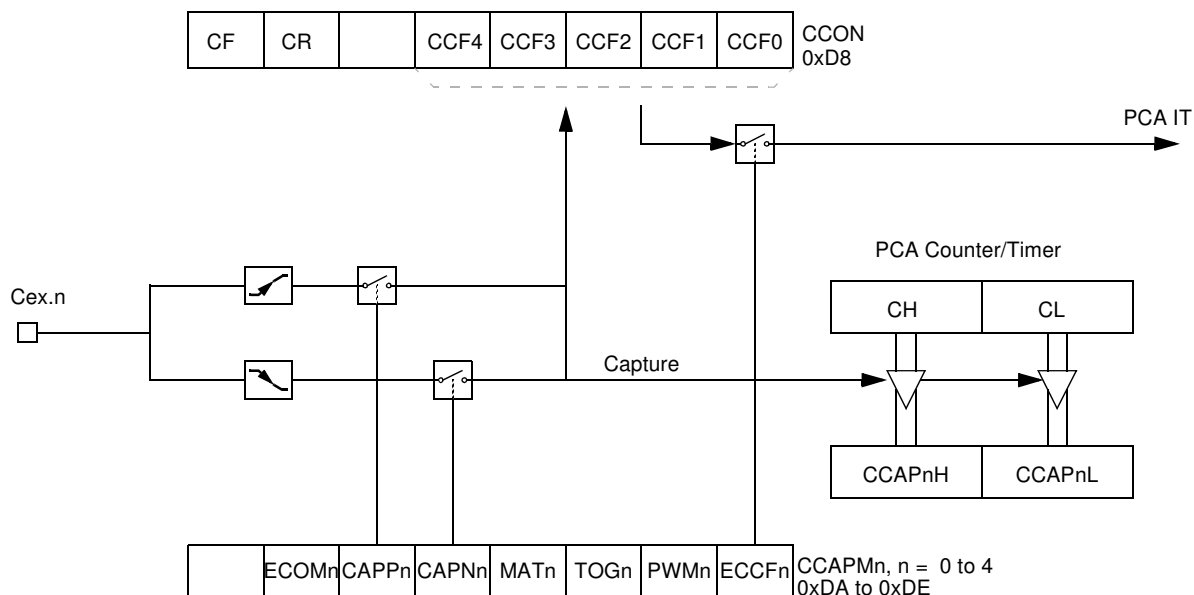
Figure 3. PCA Capture Mode
