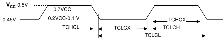
Figure 42. External Clock Drive Waveforms
