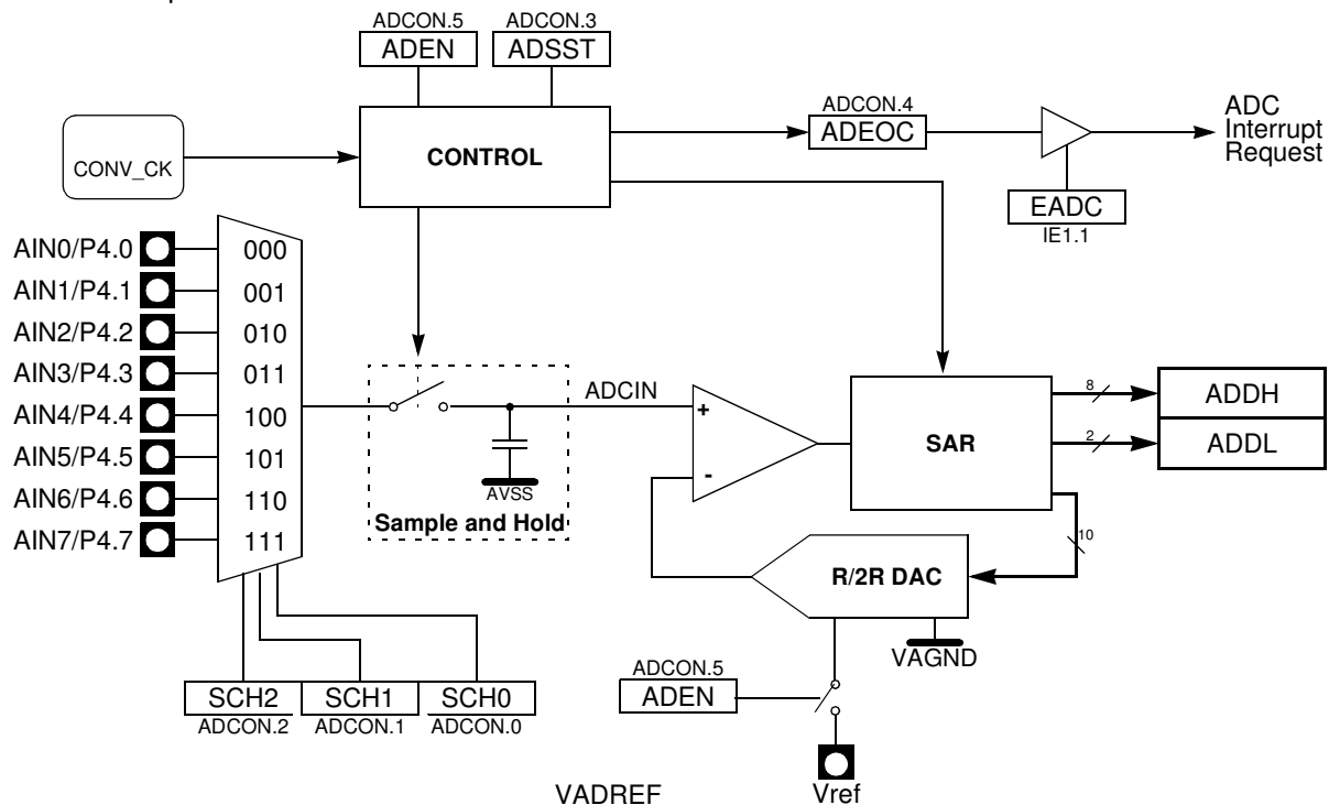
Figure 1. ADC Description
