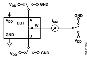
Figure 41. Common-Mode Leakage Current
