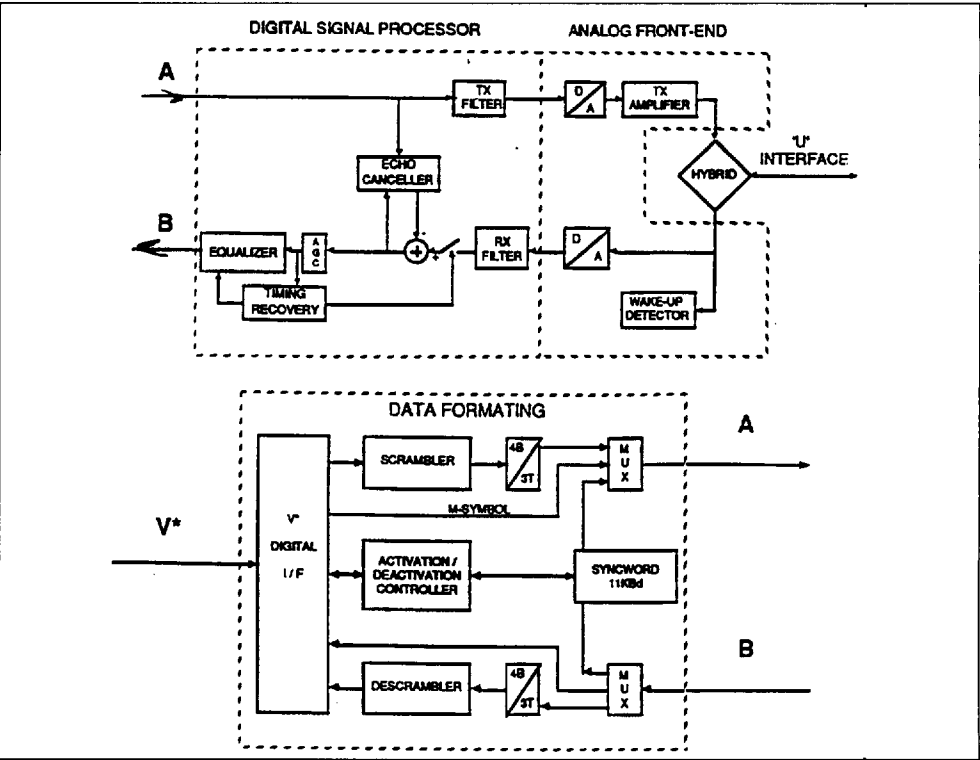
Figure 1: UIC Schematic Block Diagram
