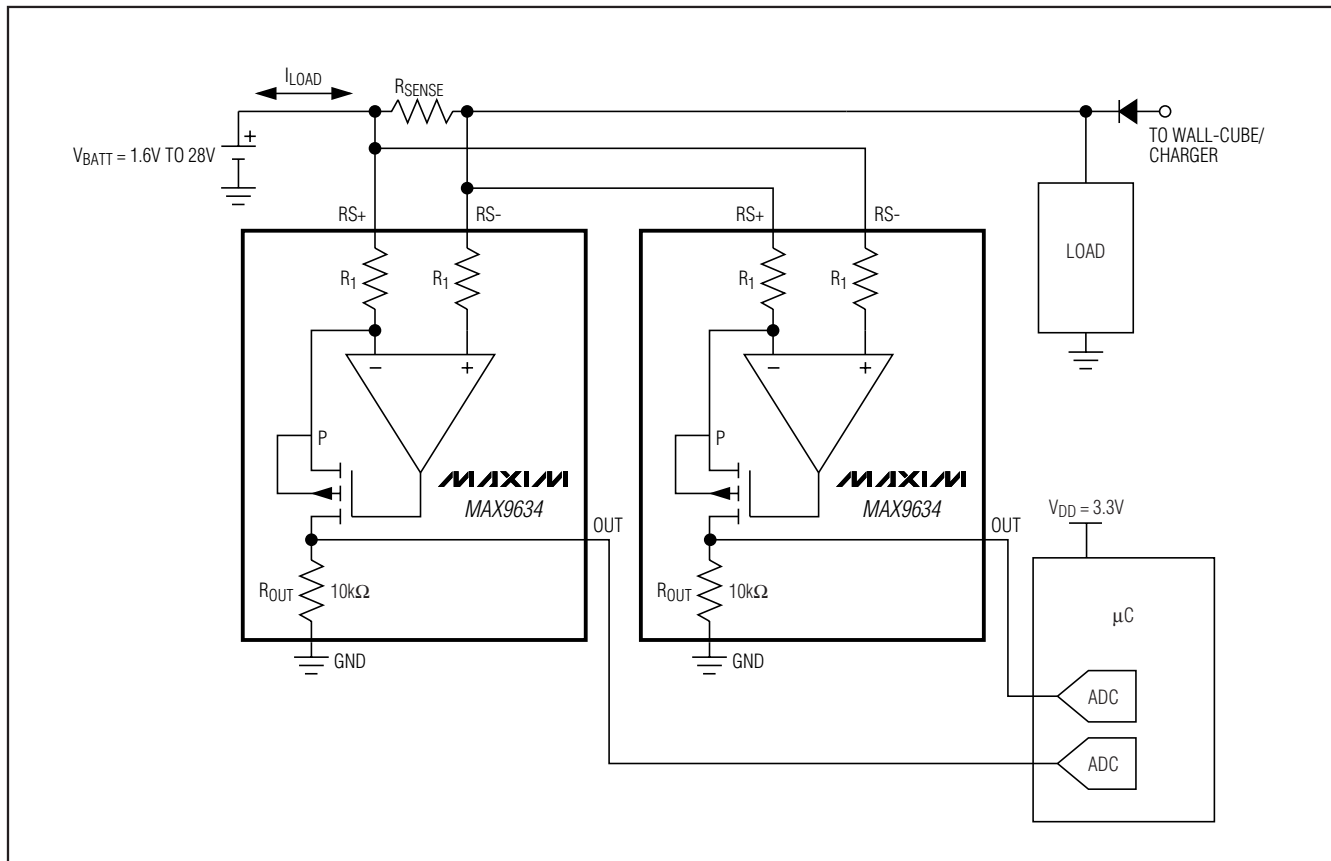
Figure 1. Bidirectional Application
