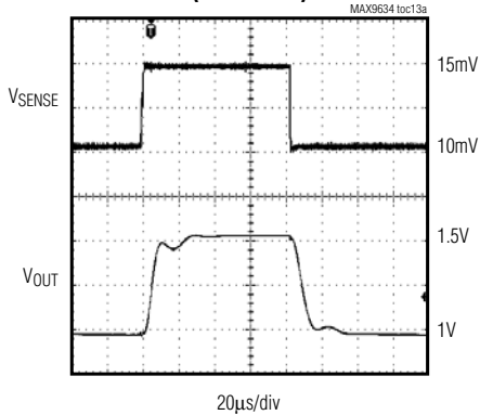
SMALL-SIGNAL PULSE RESPONSE (GAIN = 100)
