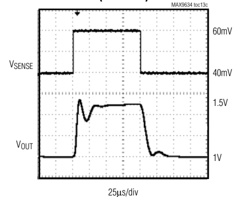
SMALL-SIGNAL PULSE RESPONSE (GAIN = 25)
