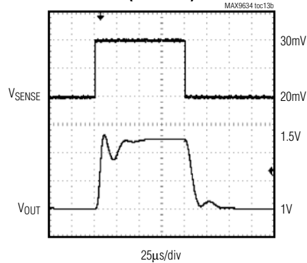
SMALL-SIGNAL PULSE RESPONSE (GAIN = 50)
