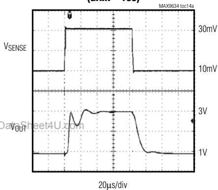
LARGE-SIGNAL PULSE RESPONSE (GAIN = 100)
