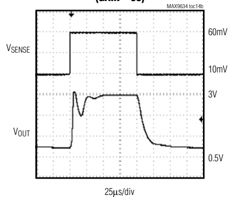
LARGE-SIGNAL PULSE RESPONSE (GAIN = 50)
