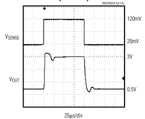
LARGE-SIGNAL PULSE RESPONSE (GAIN = 25)
