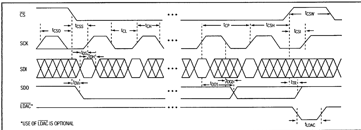
Figure 6. Detailed Serial-Interface Timing Diagram
