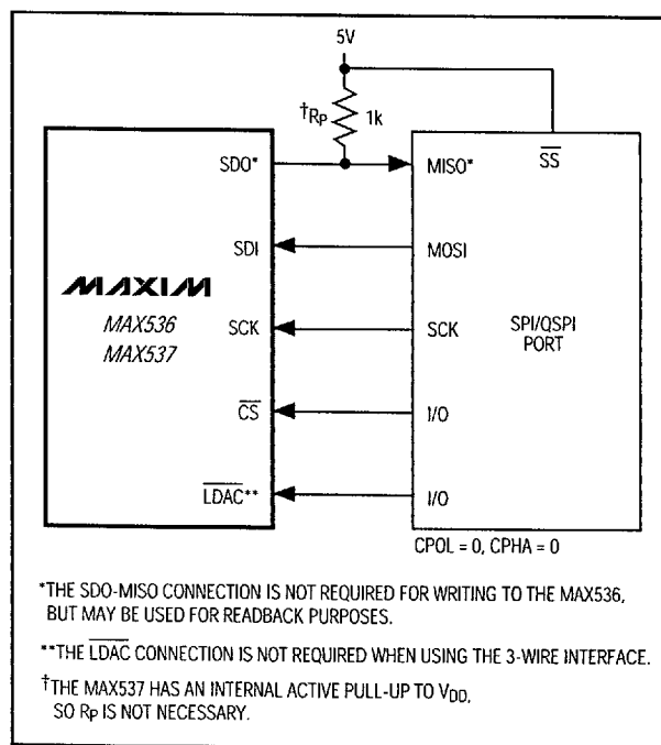
Figure 3. Connections for SPI/QSPI
