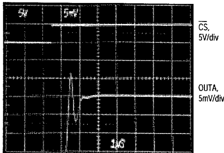
MAX537 POSITIVE FULL-SCALE SETTLING TIME (ALL BITS OFF TO ALL BITS ON)
