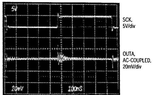
MAX537 DIGITAL FEEDTHROUGH
