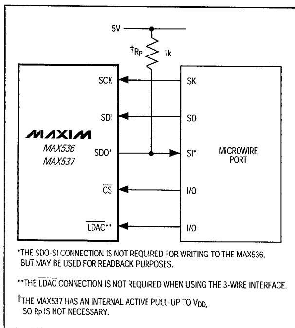
Figure 2. Connections for Microwire
