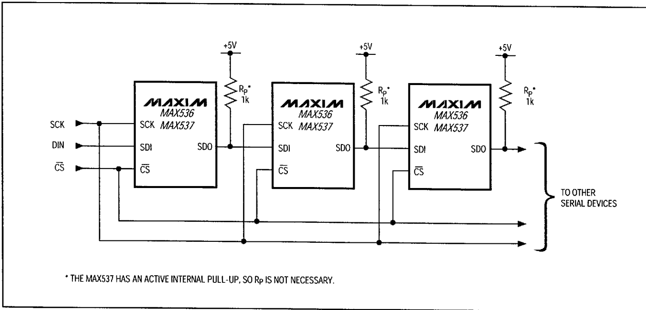
Figure 8. Daisy-Chaining MAX536/MAX537s with a 3-Wire Serial Interface
