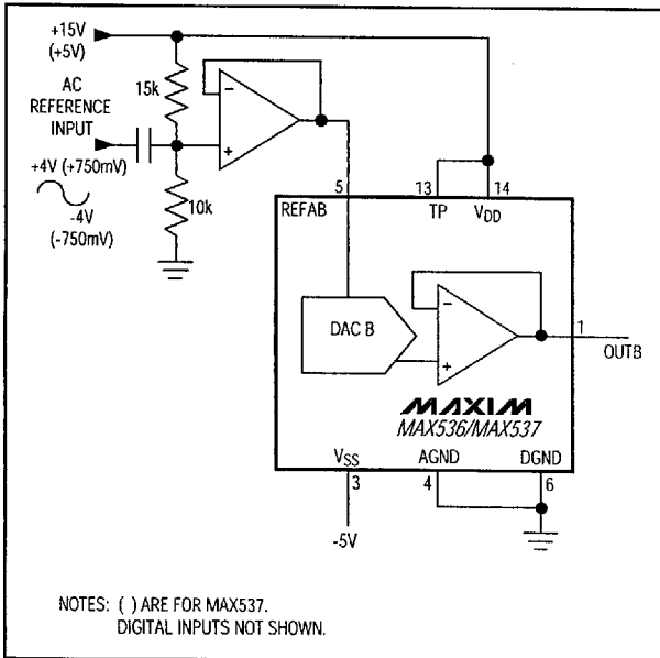
Figure 12. AC Reference Input Circuit
