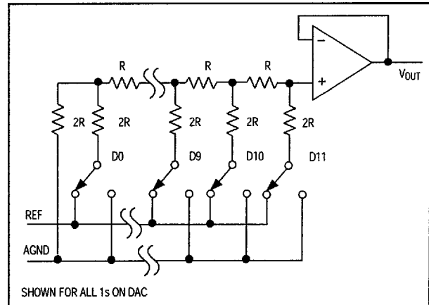
Figure 1. Simplified DAC Circuit Diagram
