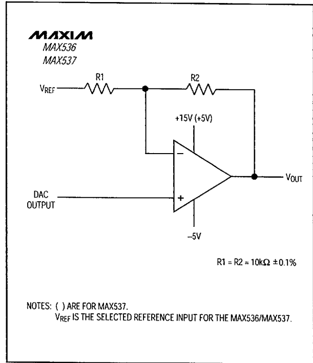
Figure 11. Bipolar Output Circuit
