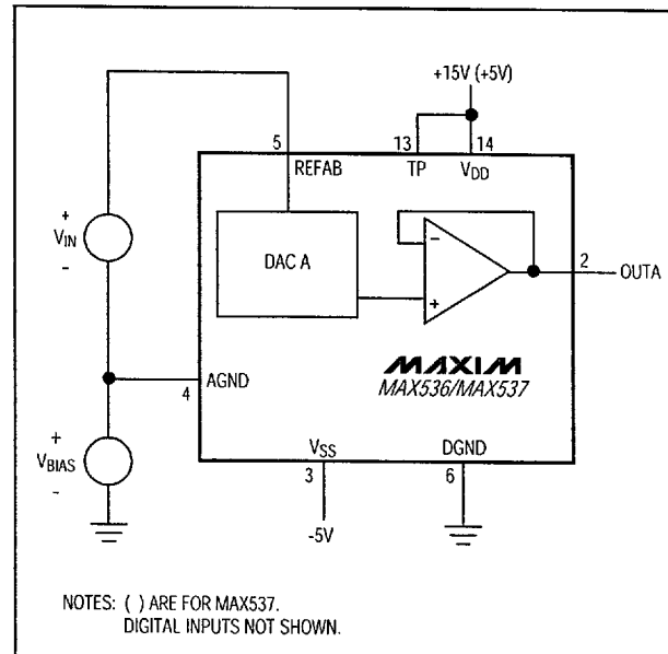
Figure 13. AGND Bias Circuit
