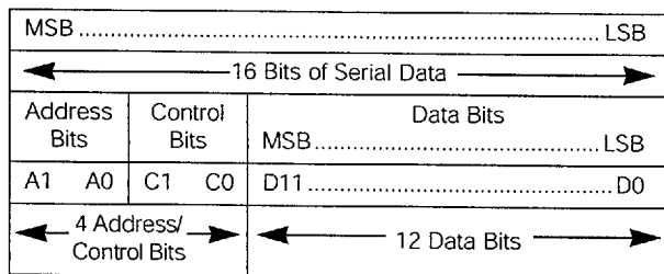
Figure 7. Serial-Data Format (MSB Sent First)
