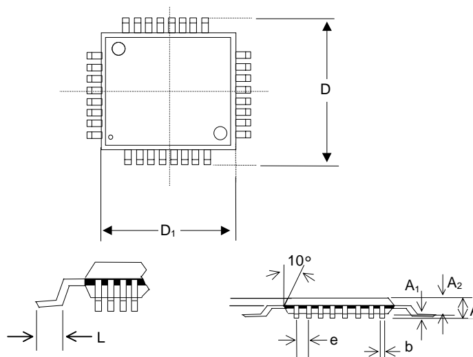
48 Pin LQFP Outline Dimensions
