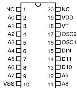
HT6032 – 20 SOP
