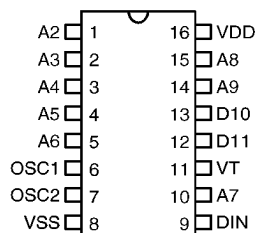
HT6035 – 16 DIP/SOP
