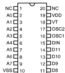
HT6034 – 20 SOP
