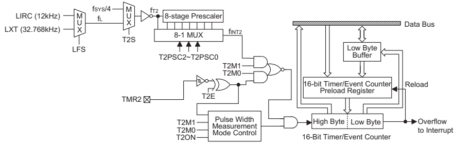
Timer/Event Counter 2
