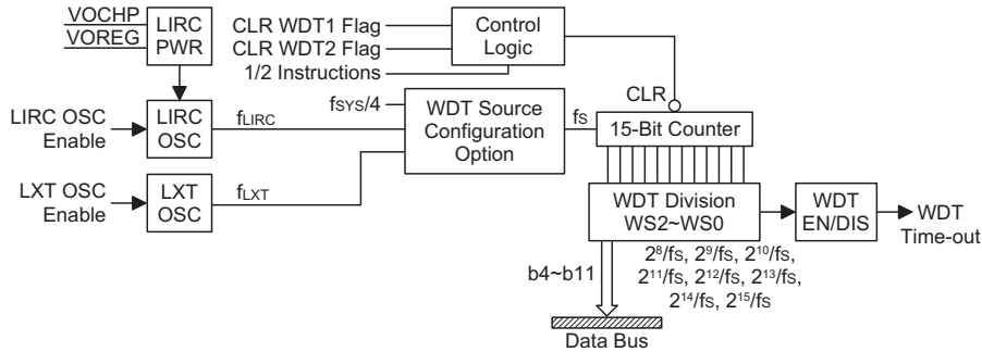
Watchdog Timer
