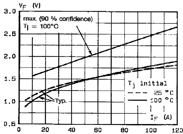
Fig. 5: Voltage drop versus forward current.
