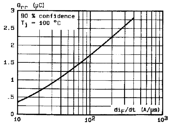
Fig. 6: Recovery charge versus di/dt.
