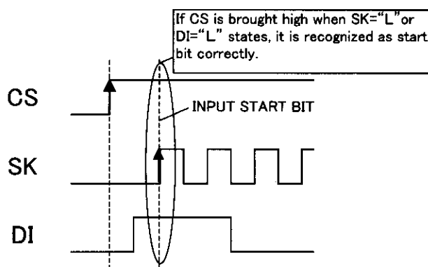
Fig.2-2 PROPER TIMING
