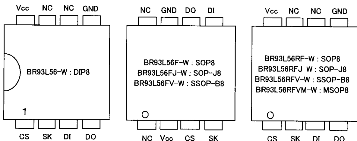
Fig.-3 Pin Configurations
