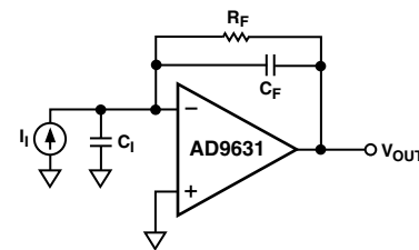
Figure 5. Transimpedance Configuration
