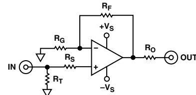
Noninverting Configuration
