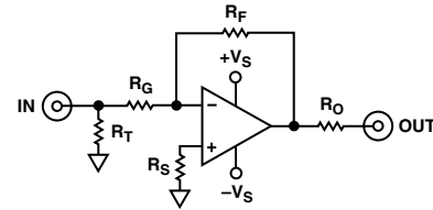
Inverting Configuration
