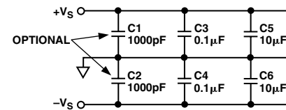
Supply Bypassing
