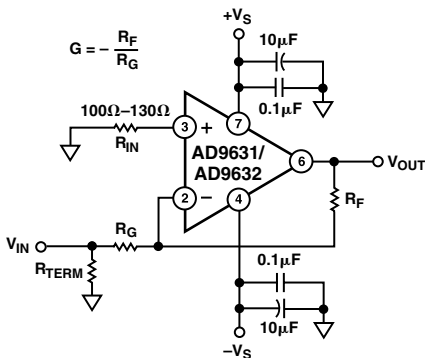
Figure 4. Inverting Operation
