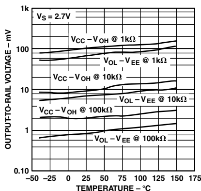
TPC 43. Output-to-Rail Voltage vs. Temperature
