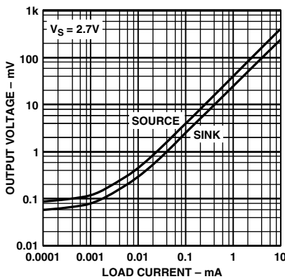
TPC 7. Output Voltage to Supply Rail vs. Load Current at 2.7 V
