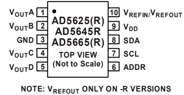
Pin Configuration (10-pin)
