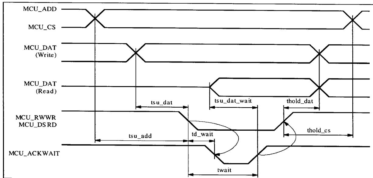
Figure 18 : MCU_MOTEL is Tied to '0'
