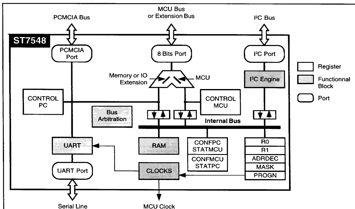
Figure 2 : Chip Block Diagram
