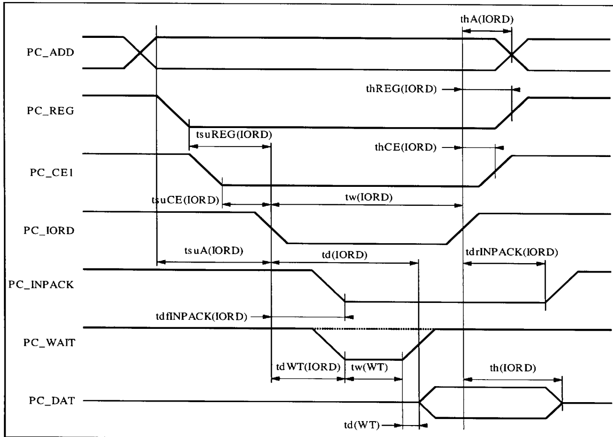
Figure 15 : Read Timing Diagram
