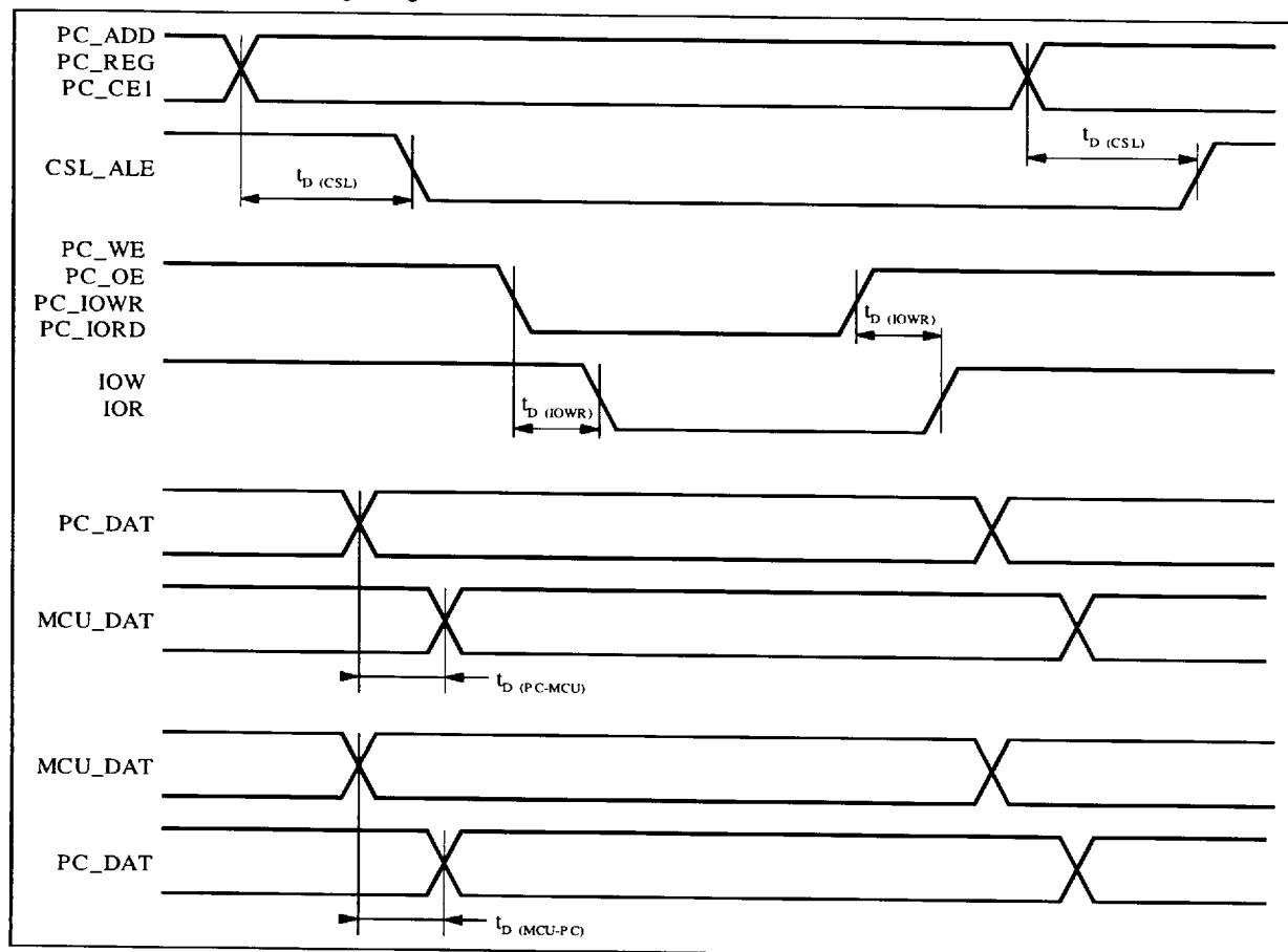
Figure 21 : Transfer Timing Diagram
