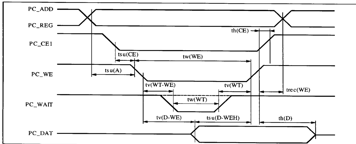
Figure 12 : Write Timing Diagram
