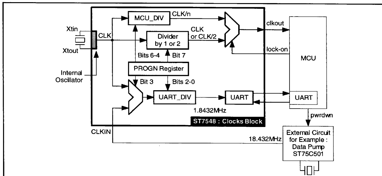
Figure 3 : Theoretical Schematic
