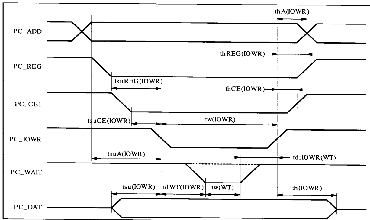
Figure 16 : Write Timing Diagram
