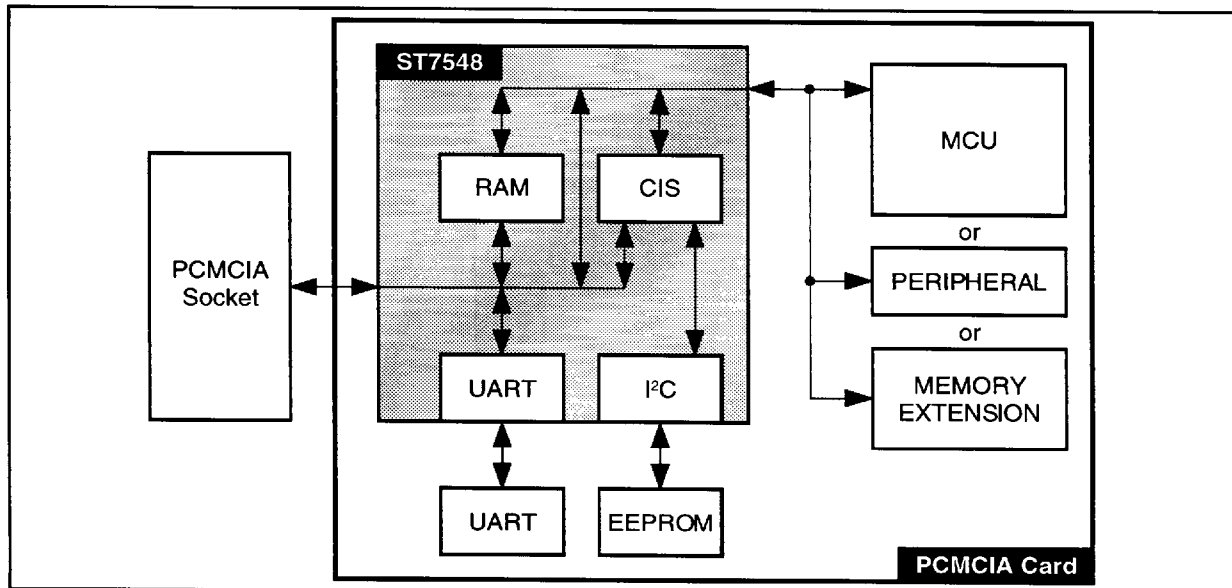
Figure 1 : Simplified Block Diagram of the Data Flows Allowed by the Chip
