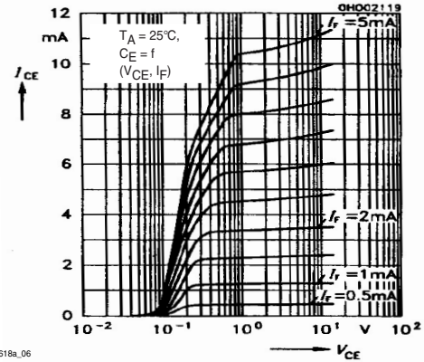
Figure 8. Output Characteristics
