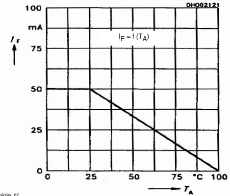
Figure 9. Permissible Forward Current Diode
