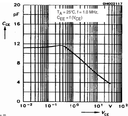
Figure 7. Transistor Capacitance
