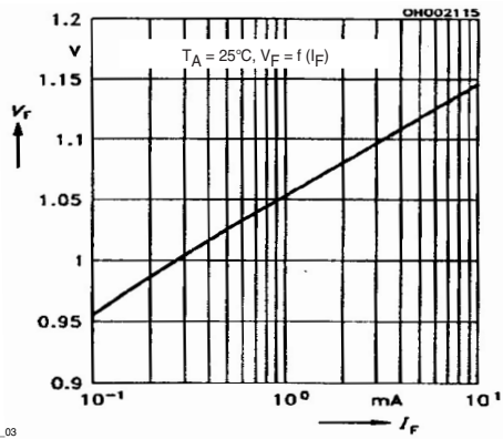
Figure 5. Diode Forward Voltage (typ.)
