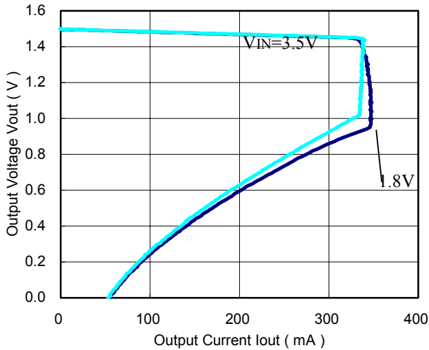
R1160N261X ECO=H
