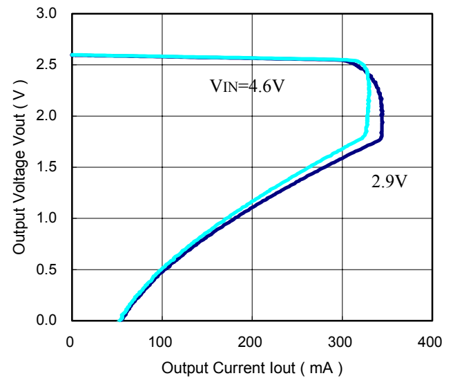
R1160N261X ECO=L
