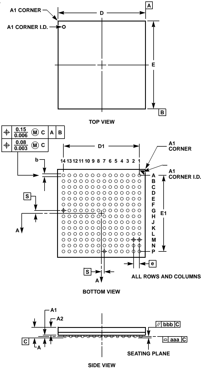
V196.15x15 196 BALL PLASTIC BALL GRID ARRAY PACKAGE
