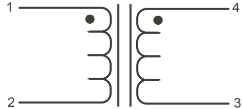
Schematic
