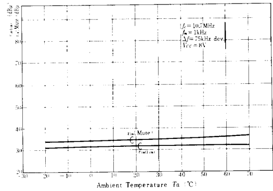
V in (Mute), V in (lim) VS. AMBIENT TEMPERATURE
