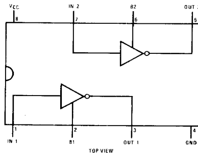
Dual-In-Line Package
