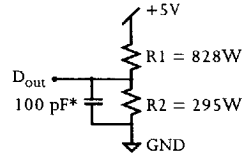
Figure B: Equivalent output load
