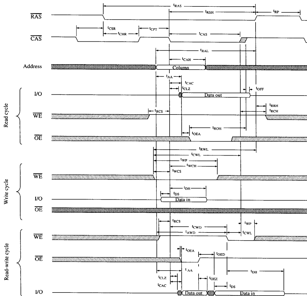
\overline{\text{CAS}} before \overline{\text{RAS}} refresh counter test waveform
