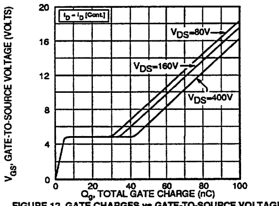
FIGURE 12, GATE CHARGES vs GATE-TO-SOURCE VOLTAGE
