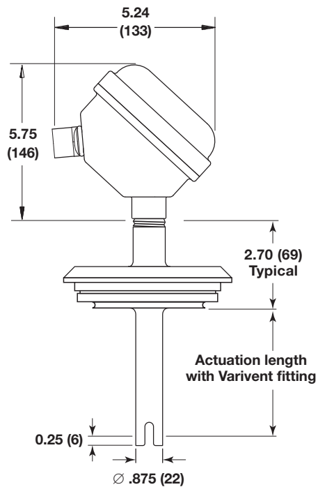
Model 960/961 with DN65 Varivent® Flange
