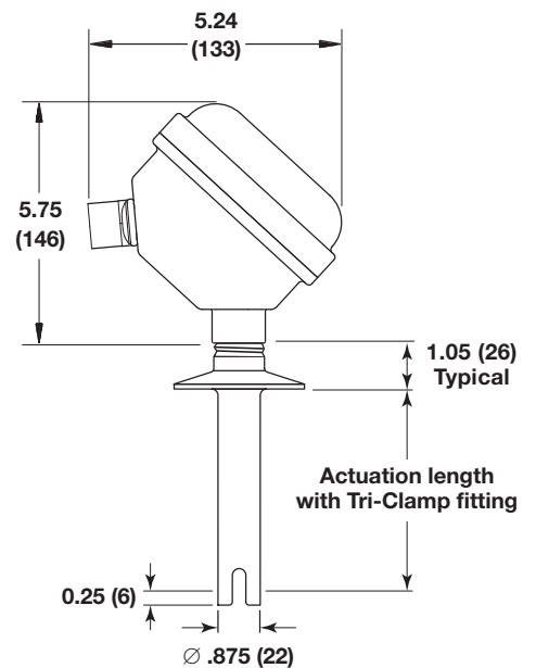
Model 960/961 with Tri-Clamp® fitting
