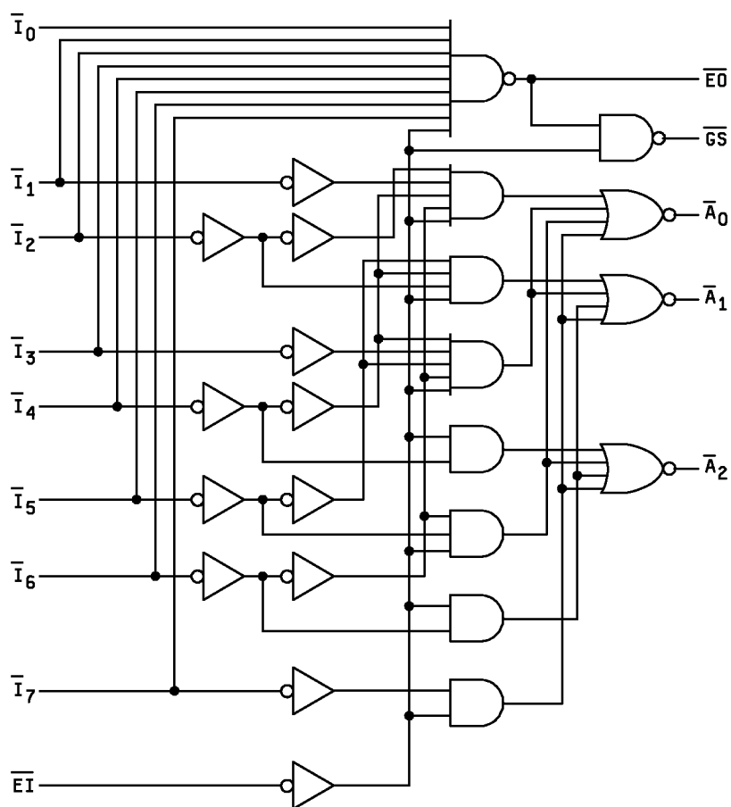
FIGURE 3. Logic diagram.
