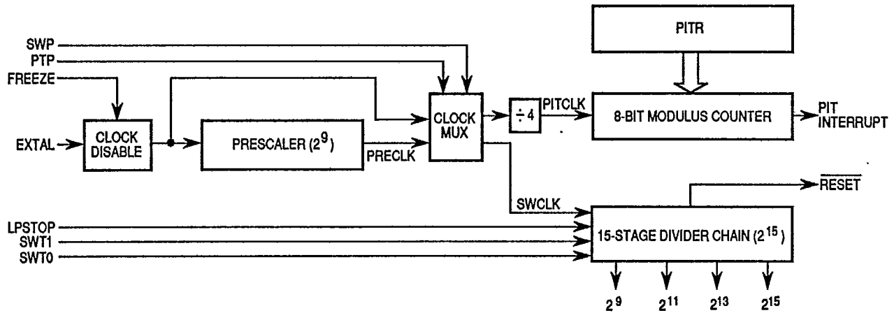
Watchdog Timer
