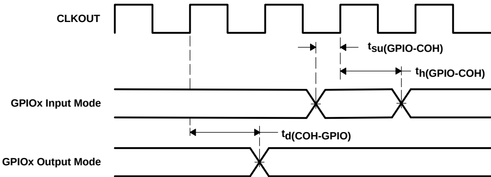
Figure 26. GPIO Timings
