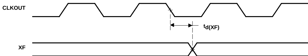
Figure 24. External Flag (XF) Timing
