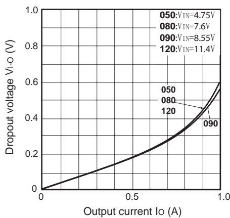
Fig.19 Dropout Voltage vs. Output Current (PQxxxRDA1SZH)
