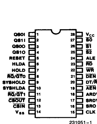
Figure 1. 82188 Pin Configuration
