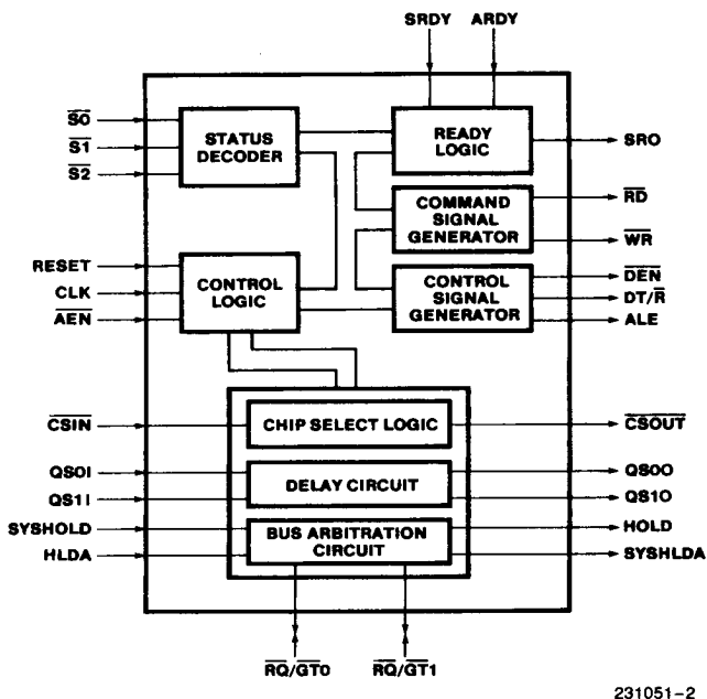
Figure 2. 82188 Block Diagram
