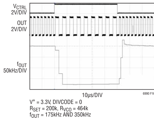
Figure 16. Settling Time
