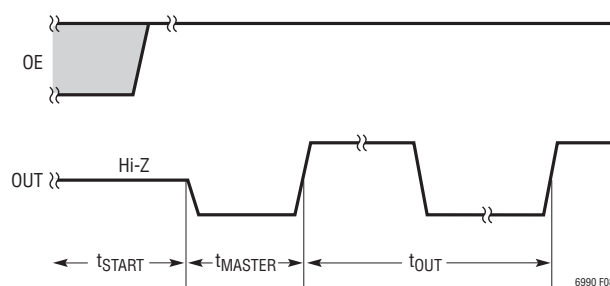
Figure 8. Start-Up Timing Diagram (OE = 1, N PIV ≥ 4, Hi-Z = 0 or 1)
